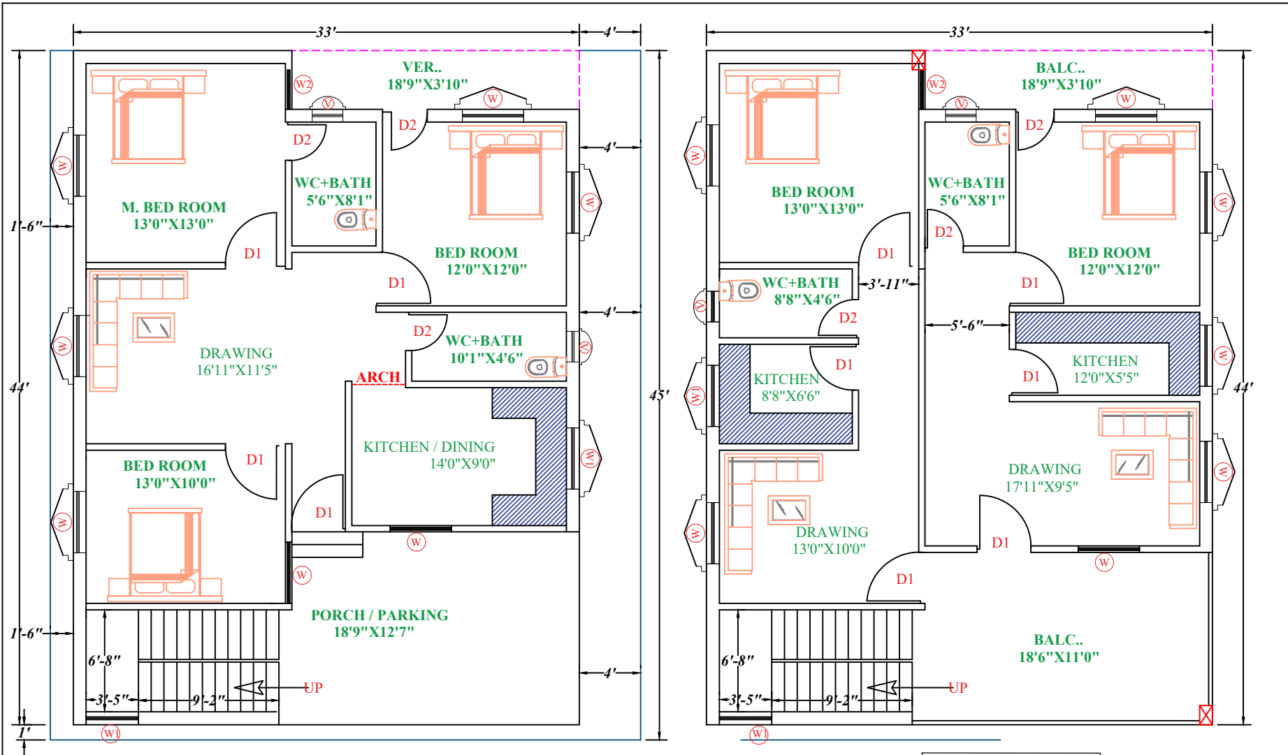
1ST & 2ND FLOOR
