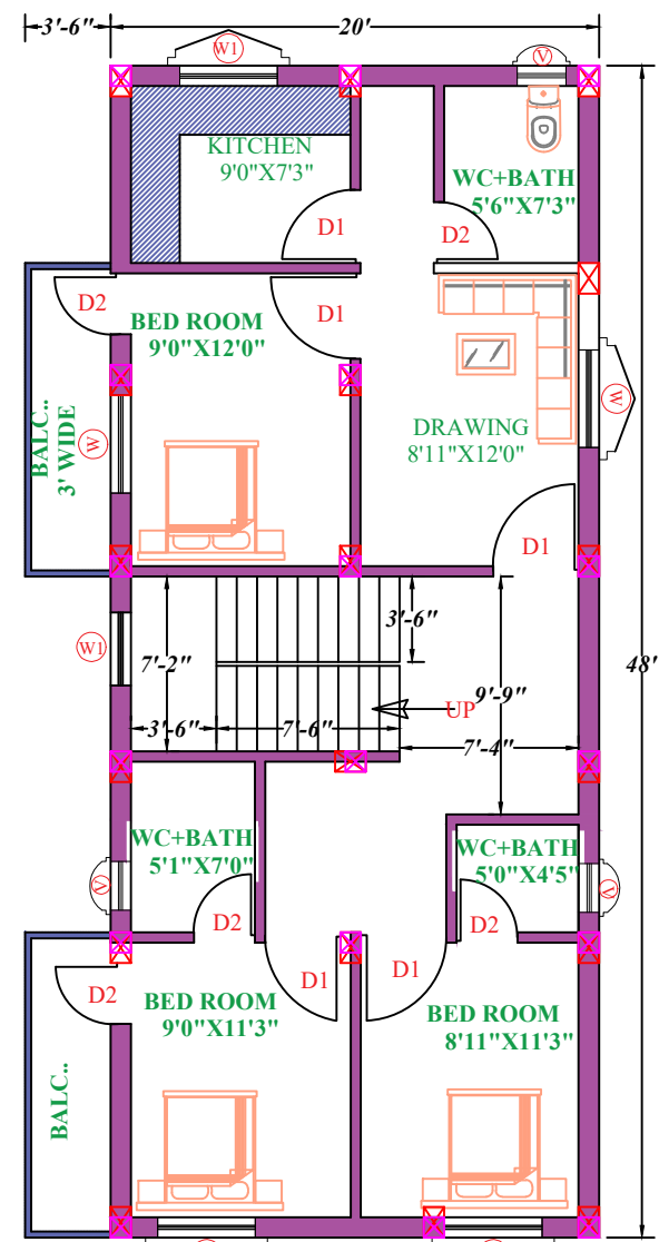
2ND, 3RD & 4TH FLOOR
