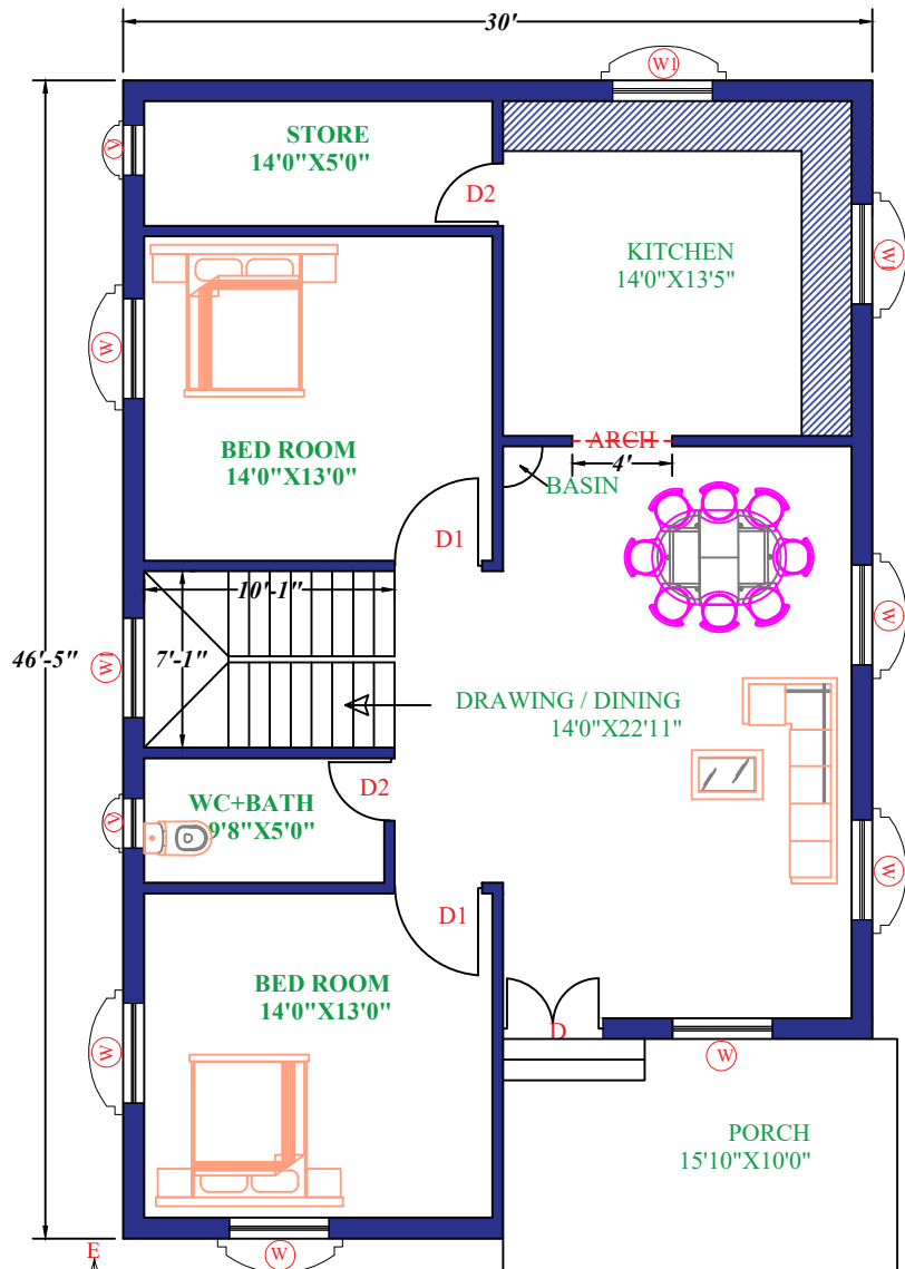
GROUND FLOOR
