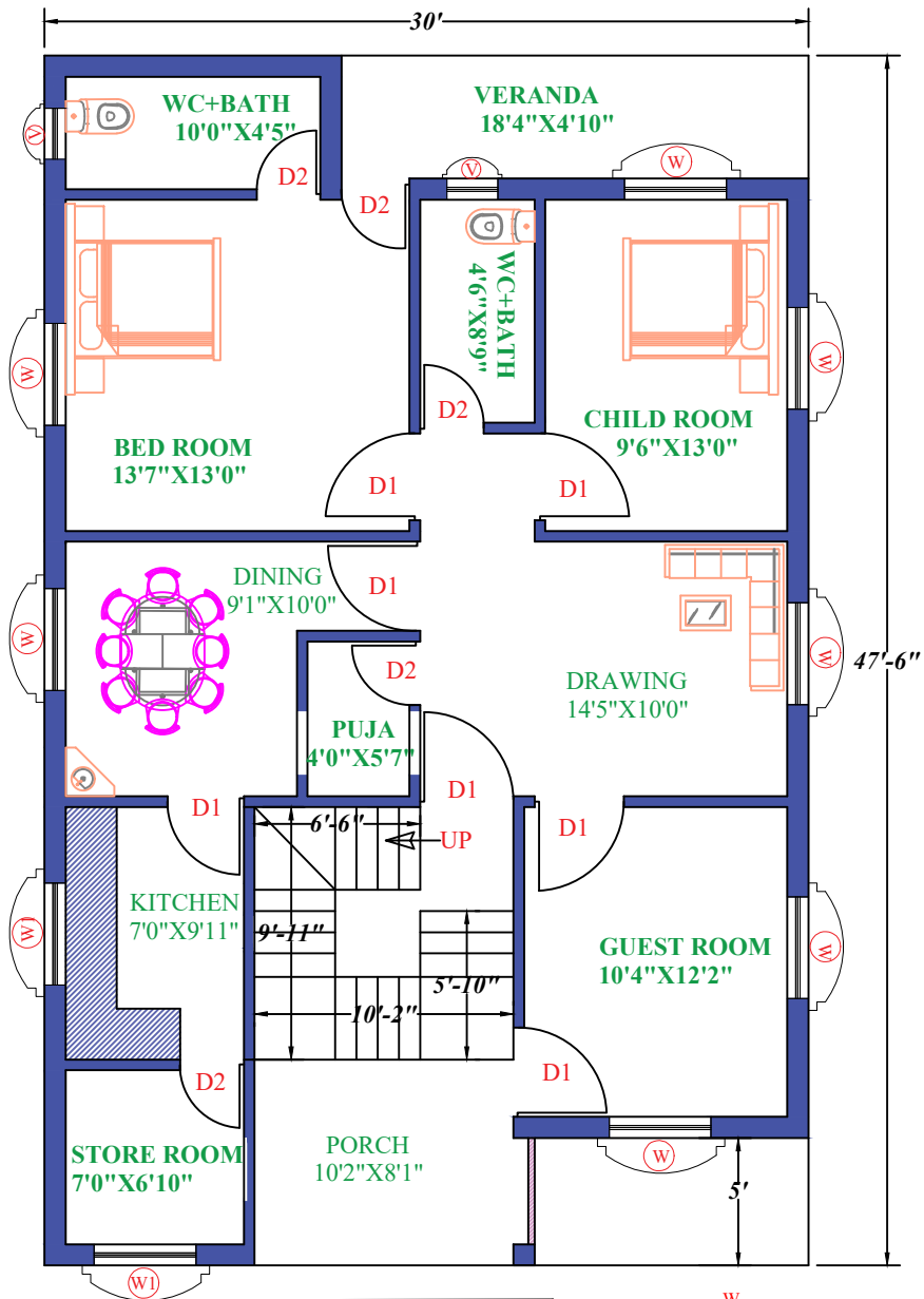
GROUND FLOOR
