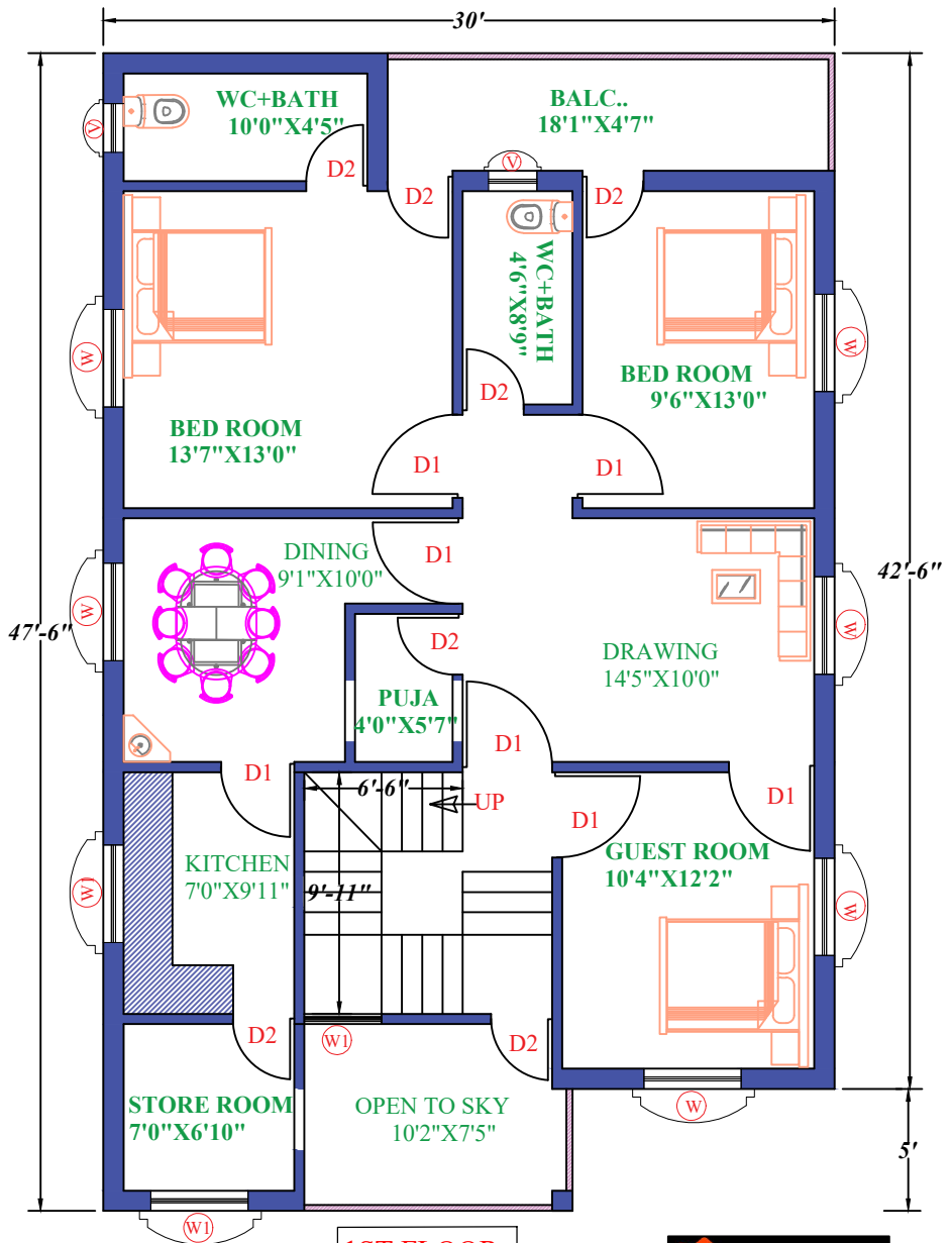
1ST FLOOR
