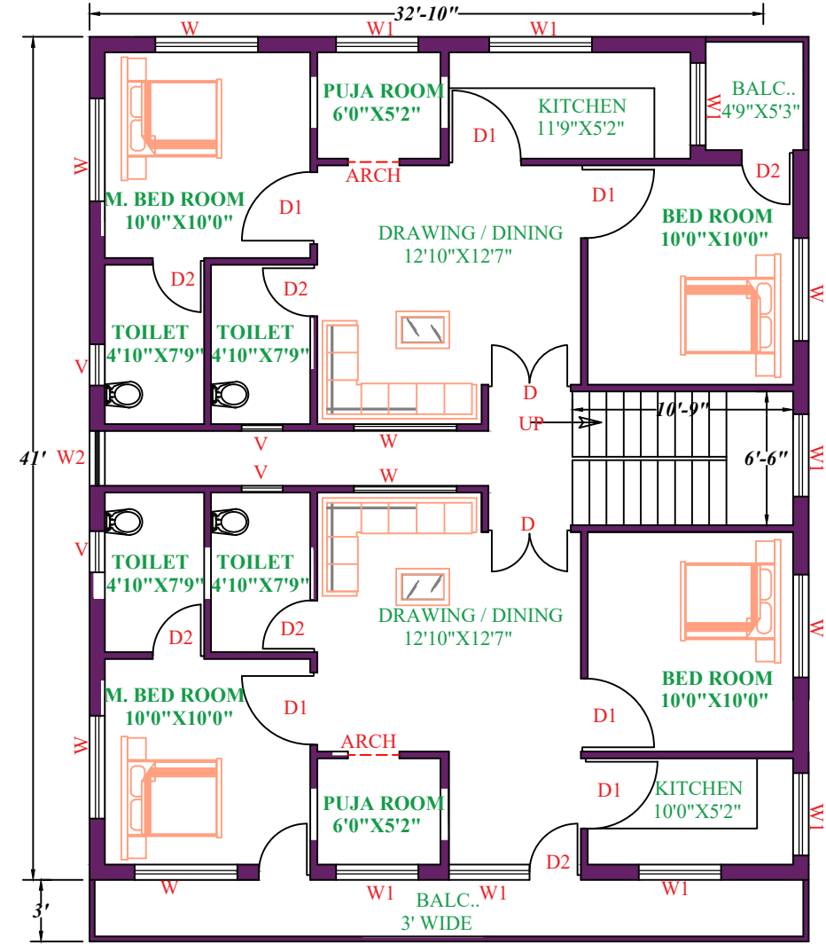
1ST FLOOR
