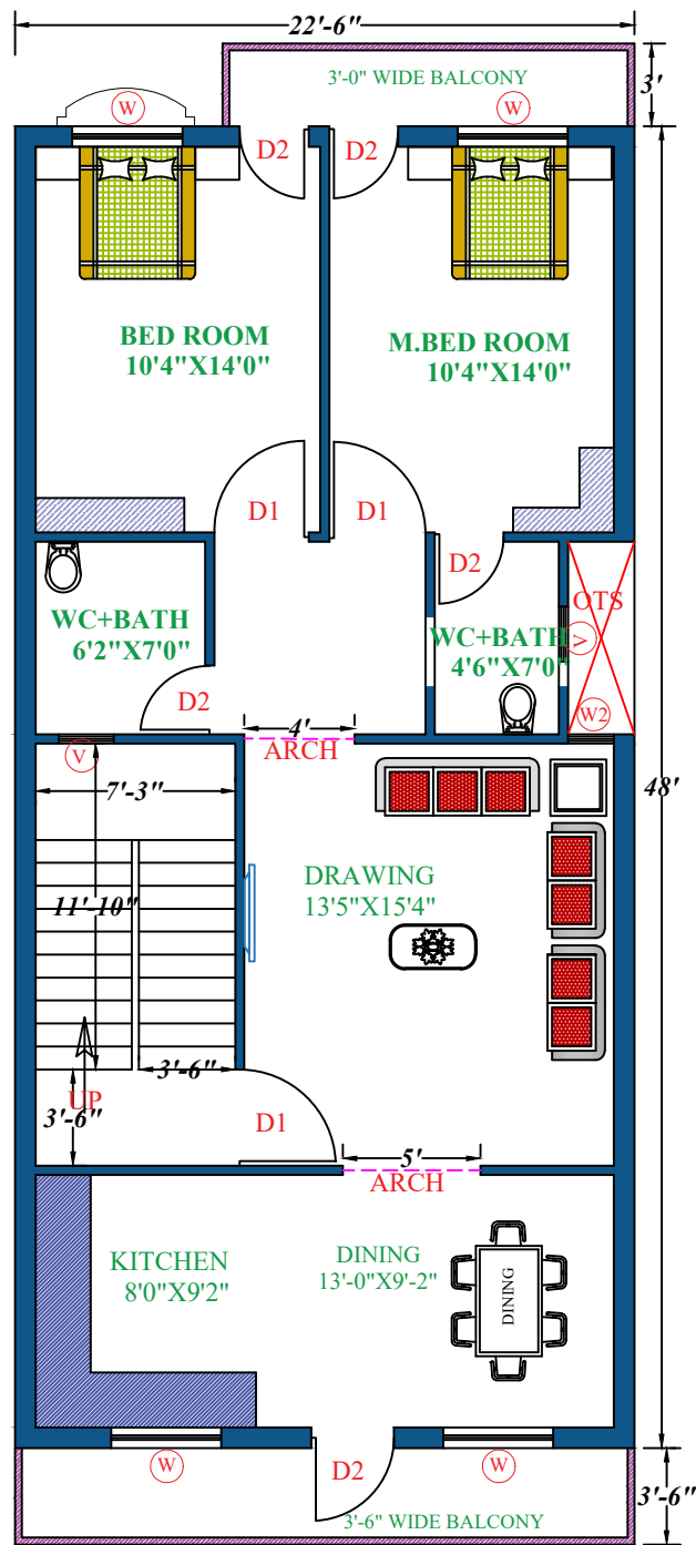
1ST, 2ND & 3RD FLOOR
