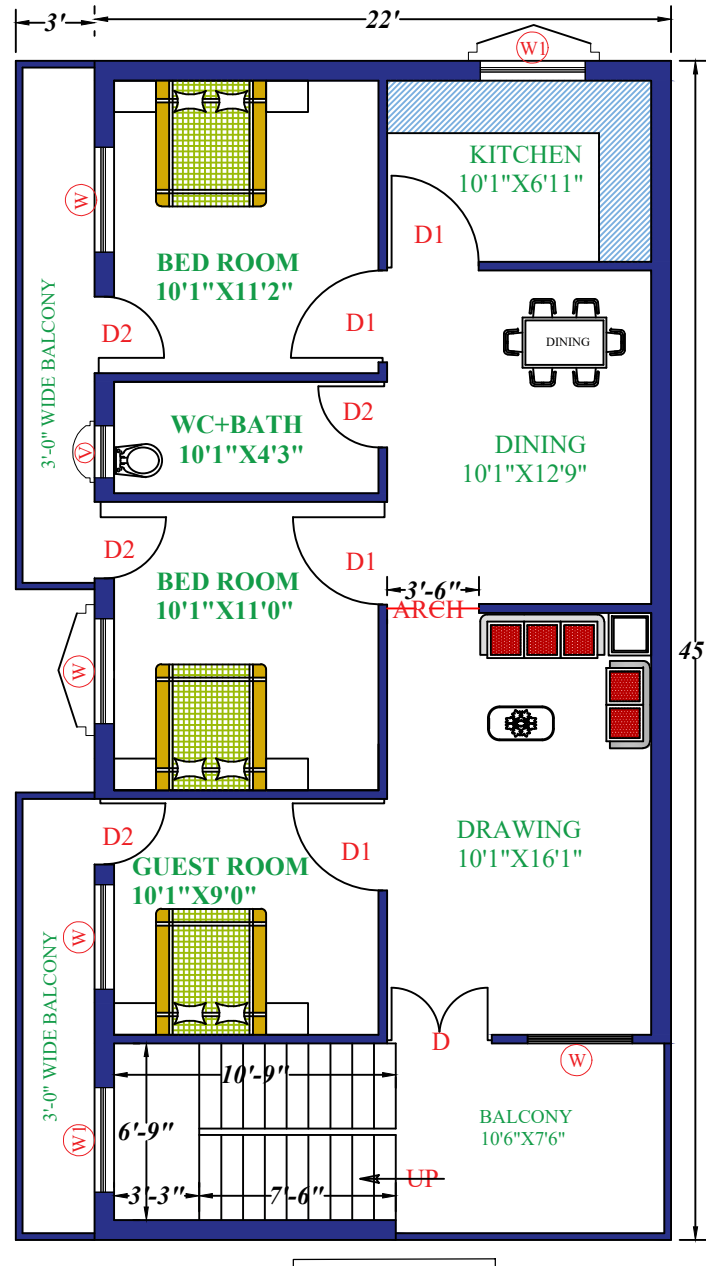
1ST FLOOR
