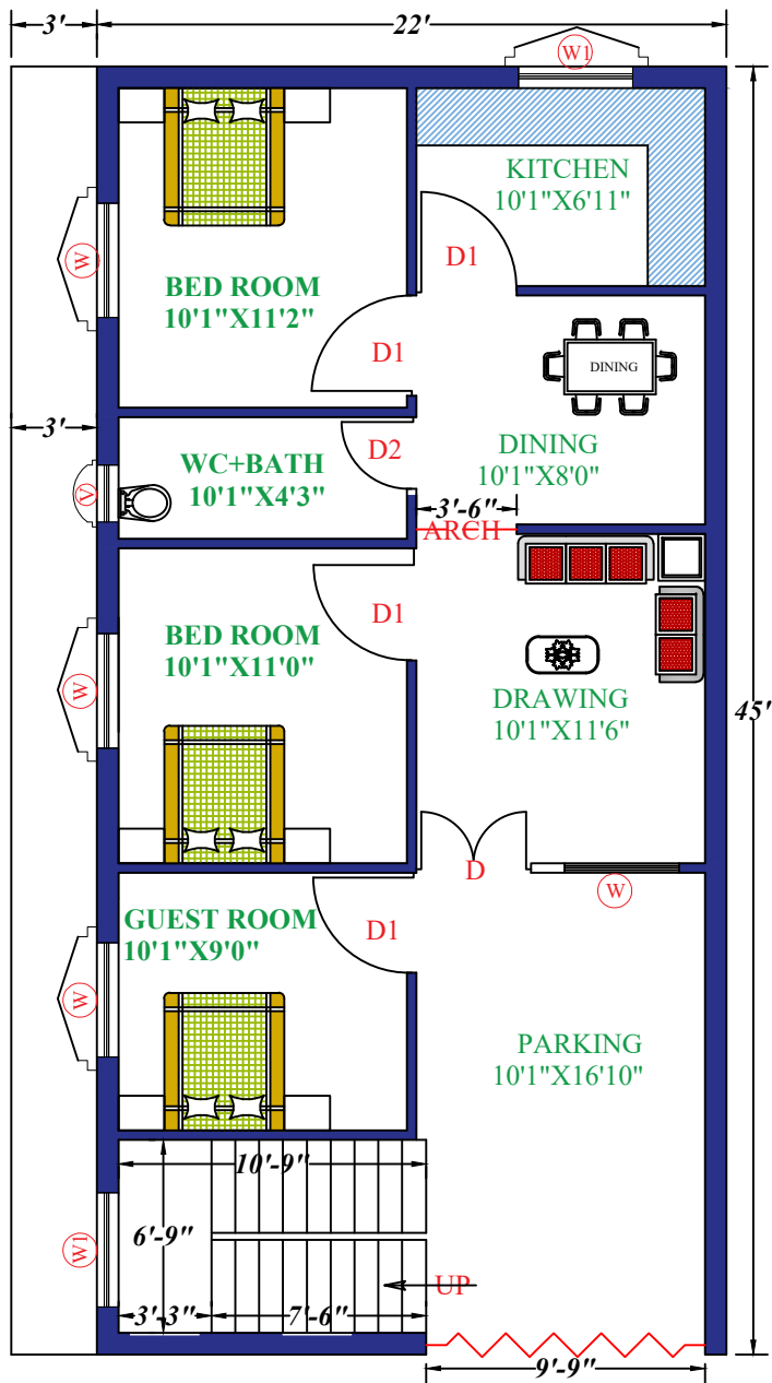
GROUND FLOOR
