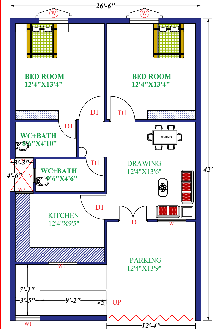
GROUND FLOOR
