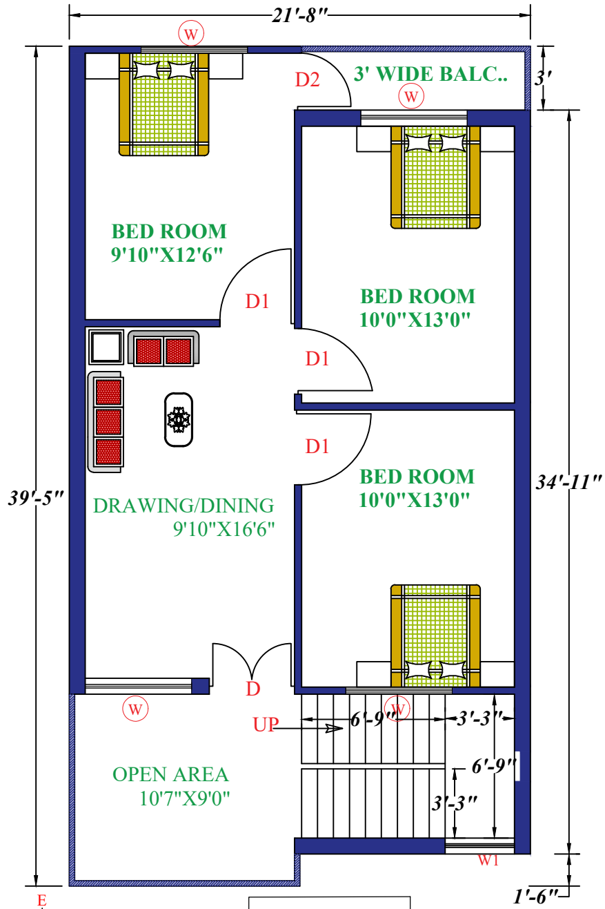
1ST FLOOR
