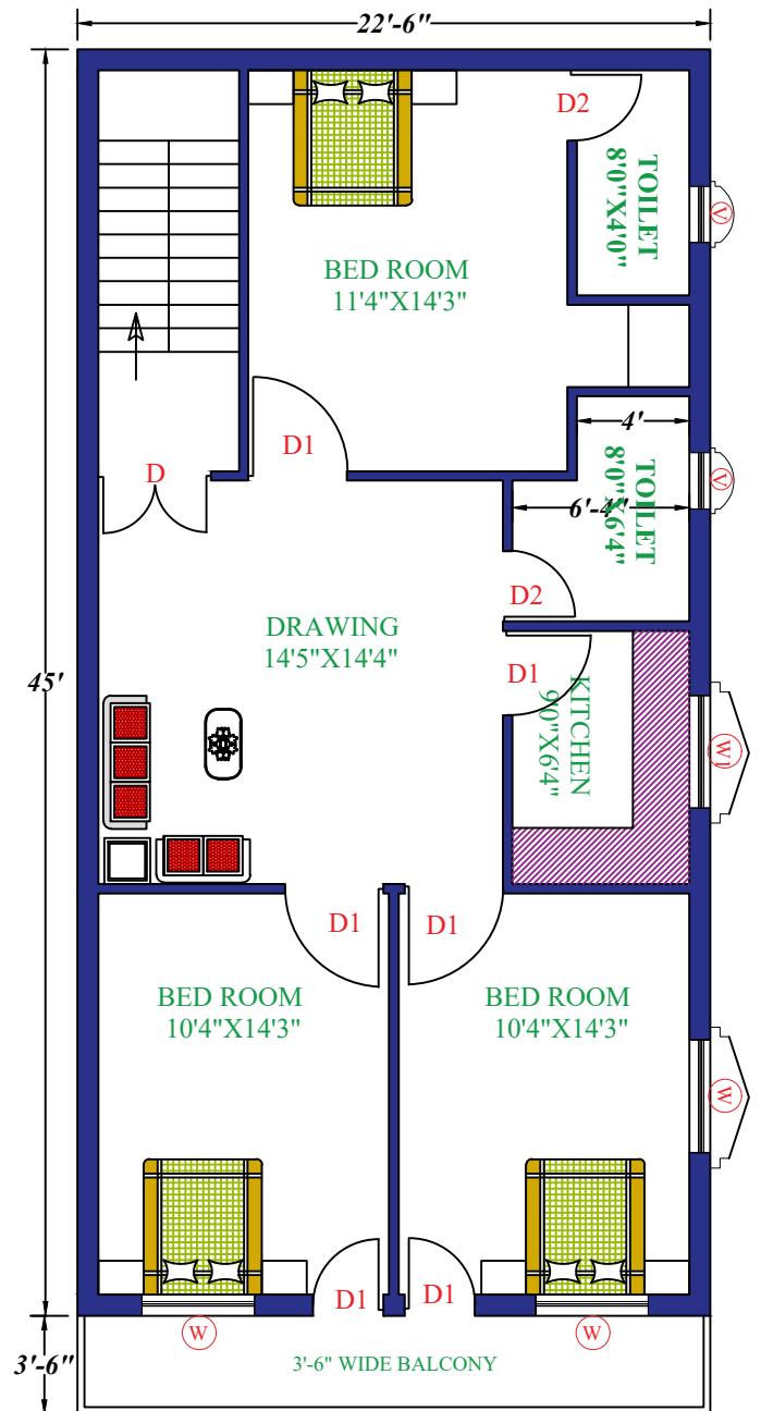
1ST FLOOR
