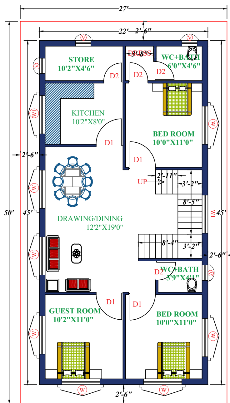
1ST FLOOR
