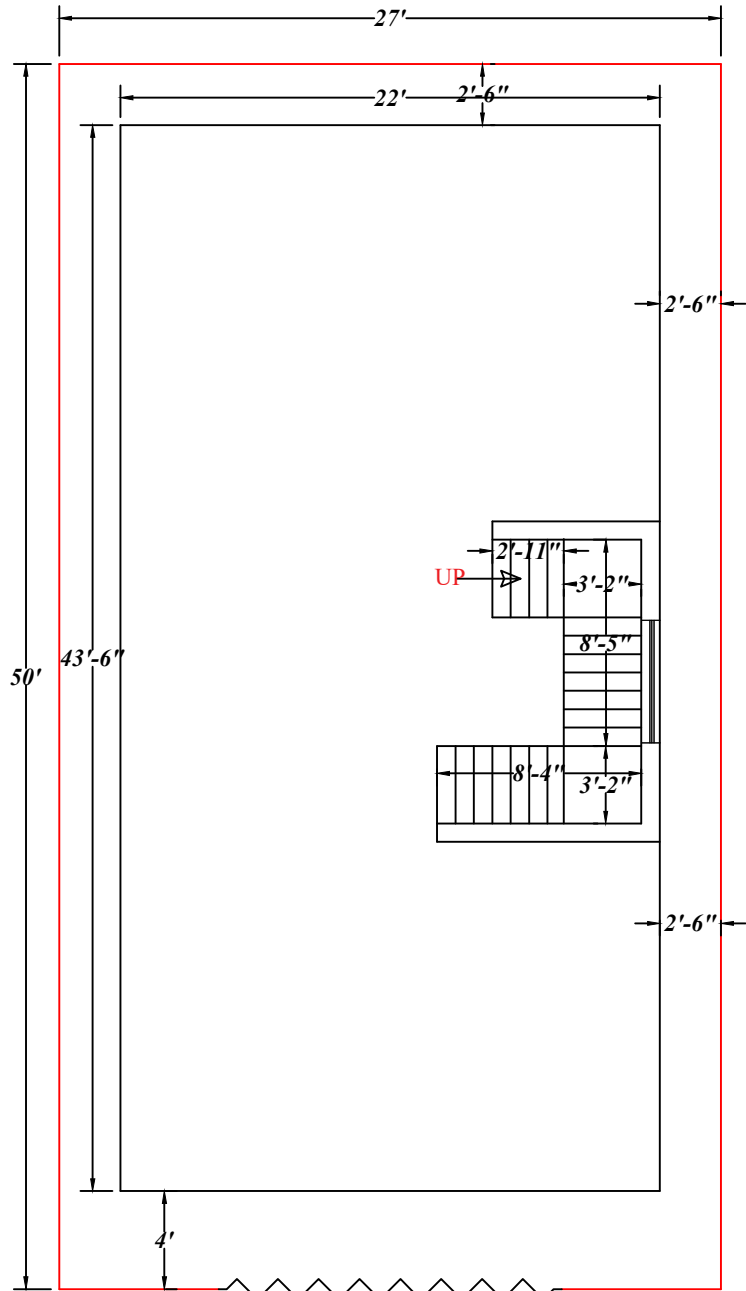
GROUND FLOOR
