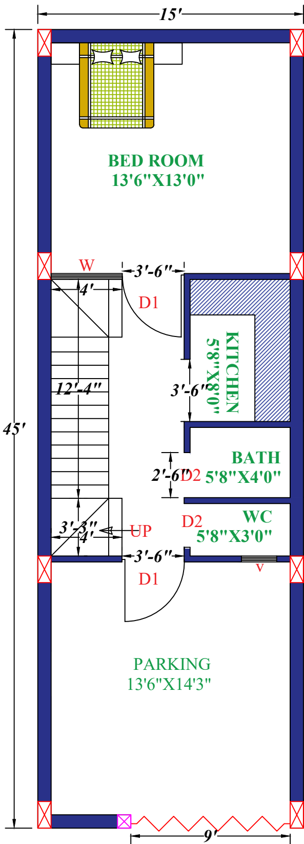
GROUND FLOOR
