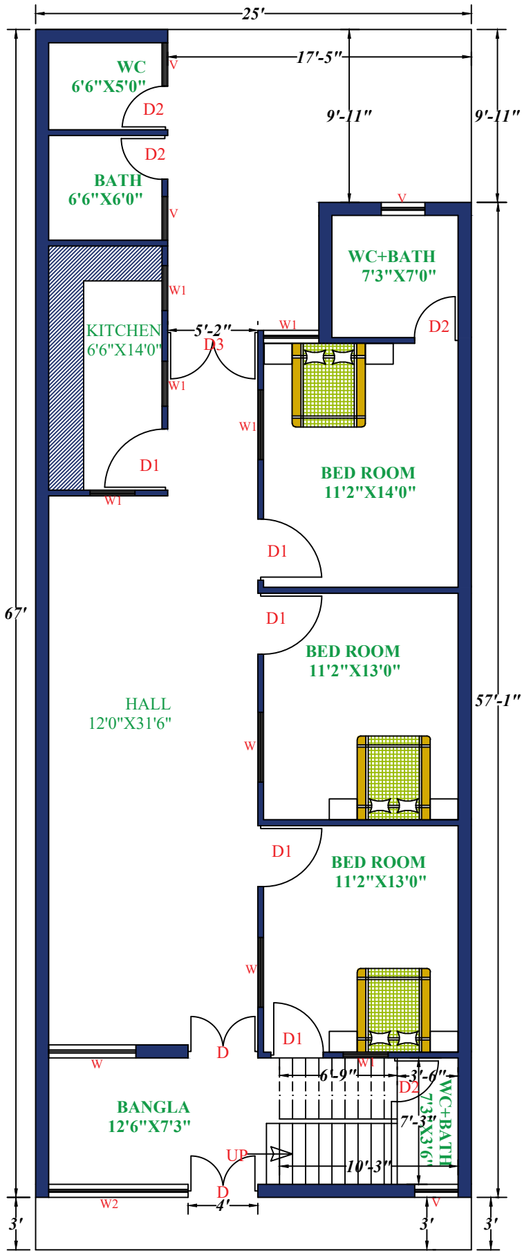
GROUND FLOOR
