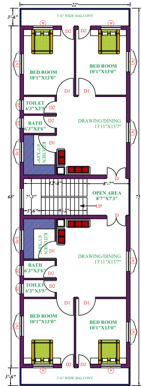
1ST & 2ND FLOOR
