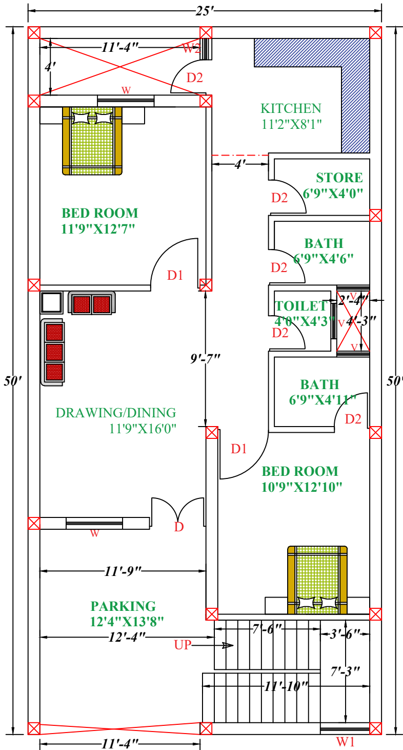
GROUND FLOOR
