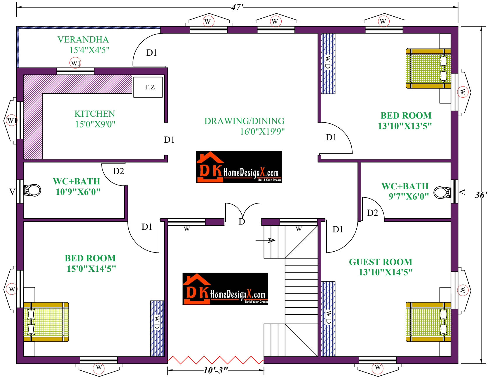
GROUND FLOOR
