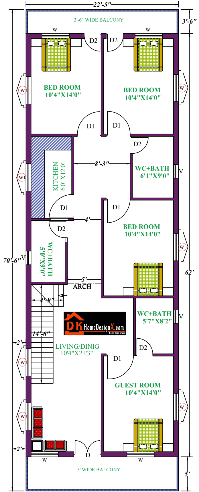
1ST FLOOR
