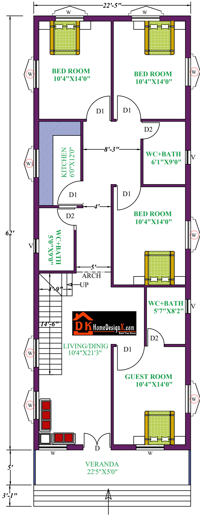
GROUND FLOOR
