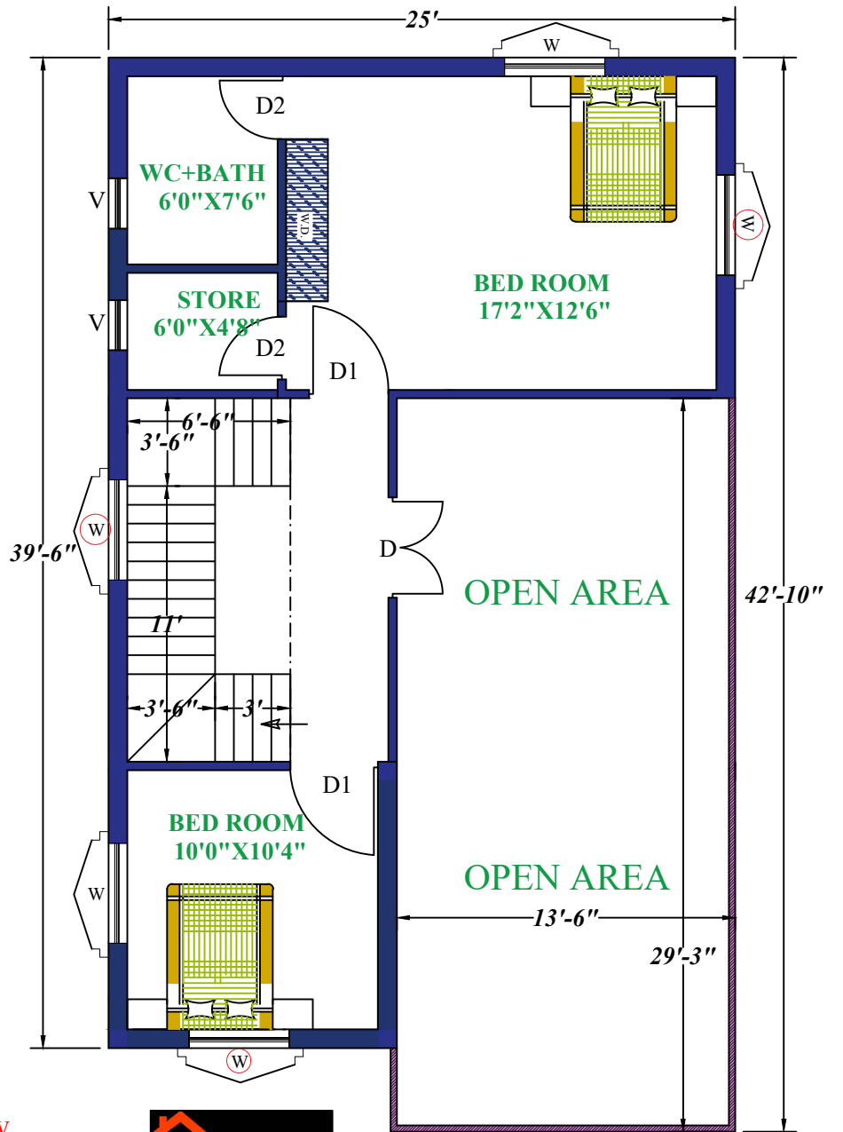
1ST FLOOR
