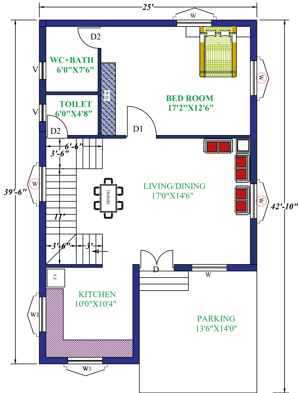
GROUND FLOOR
