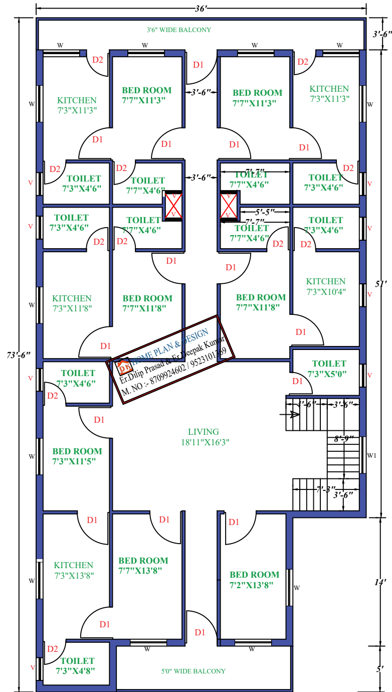
1ST FLOOR
