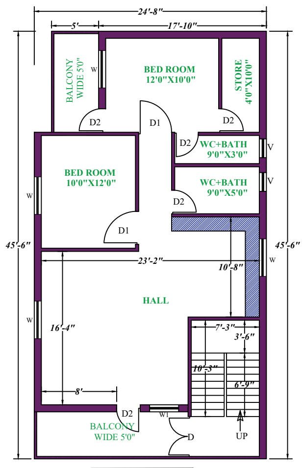
1ST & 2ND FLOOR
