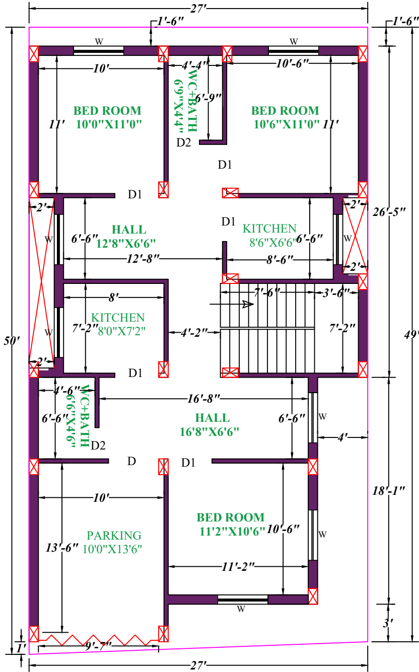
GROUND FLOOR
