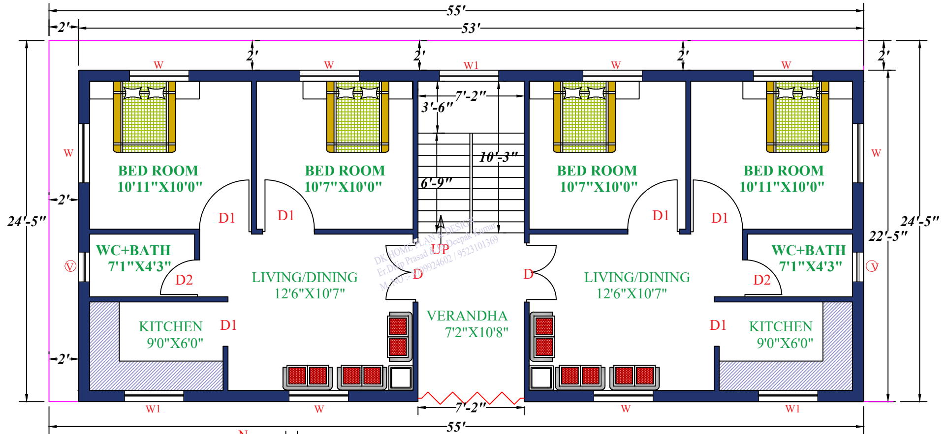
GROUND FLOOR
