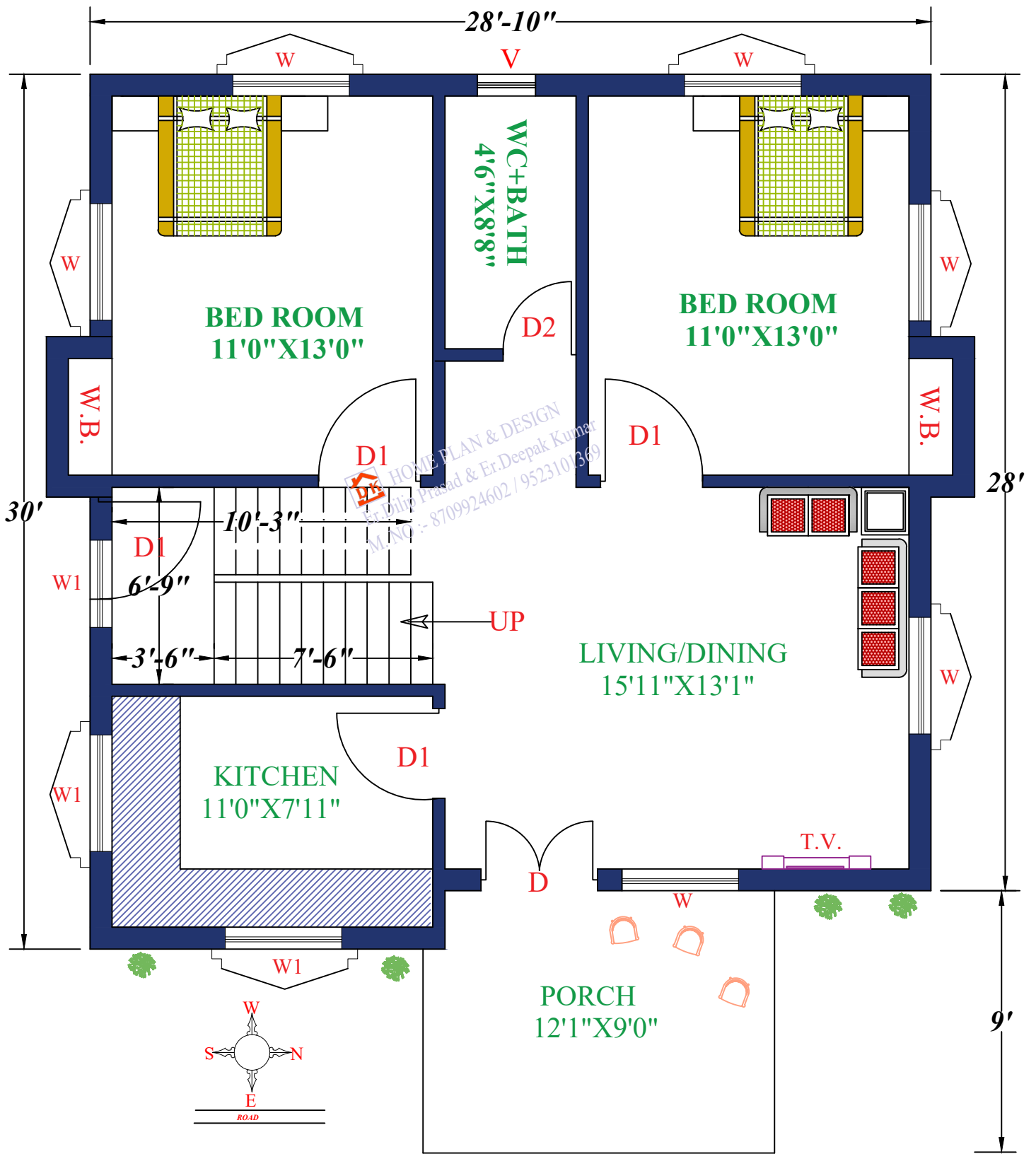
GROUND FLOOR
