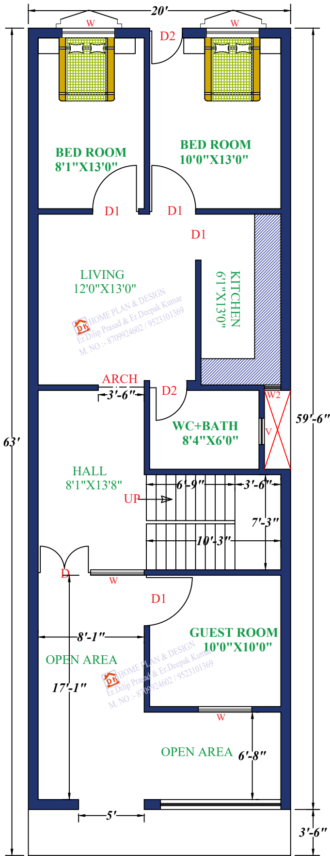
GROUND FLOOR
