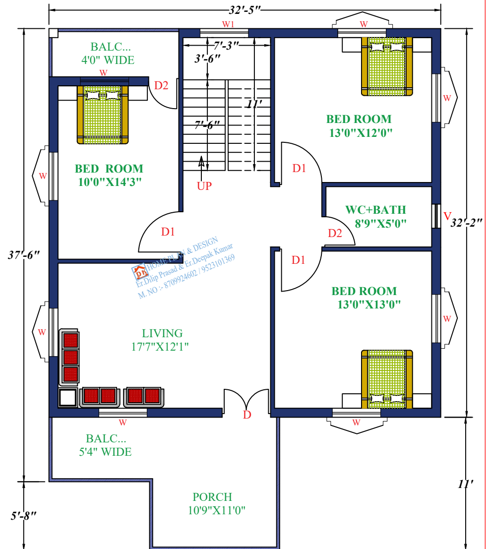
1ST FLOOR
