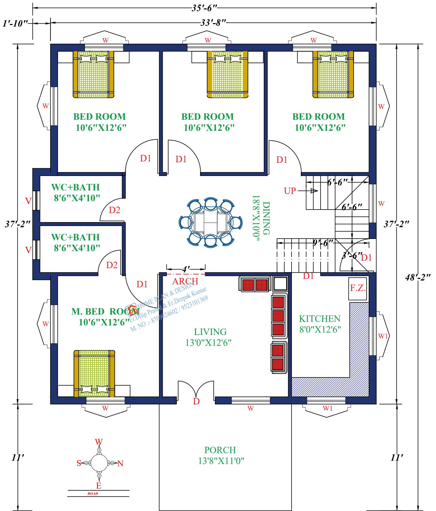
GROUND FLOOR
