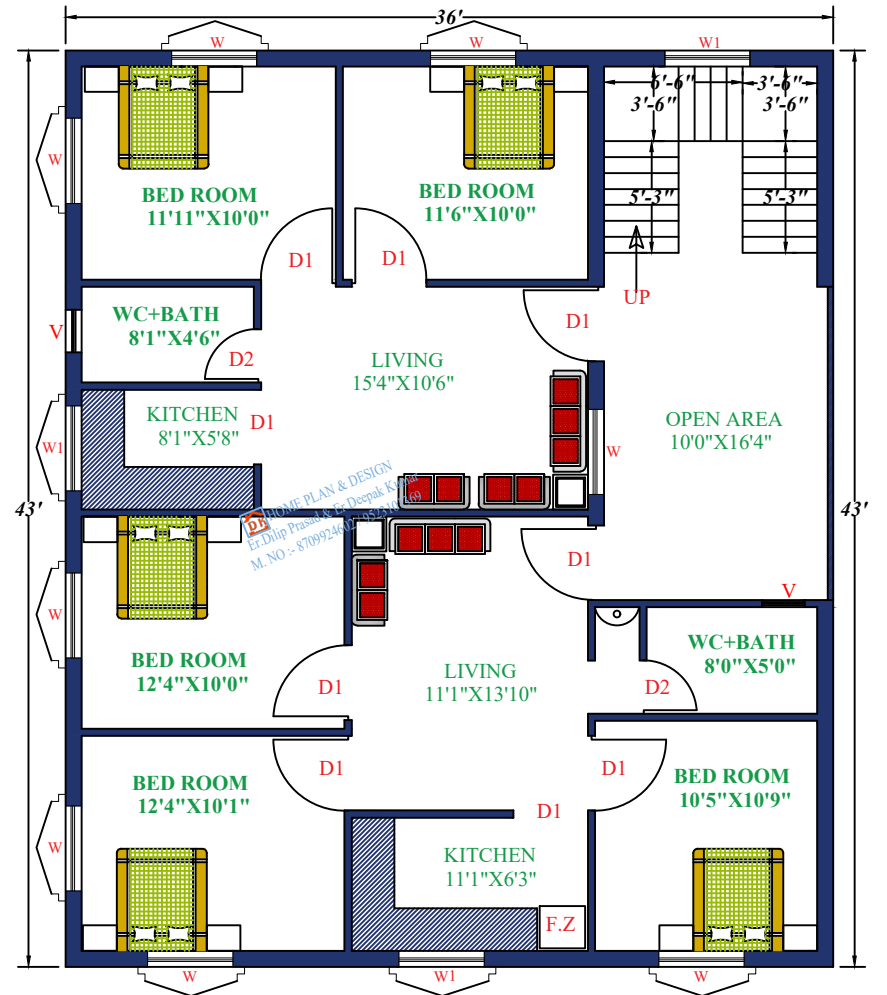
1ST FLOOR
