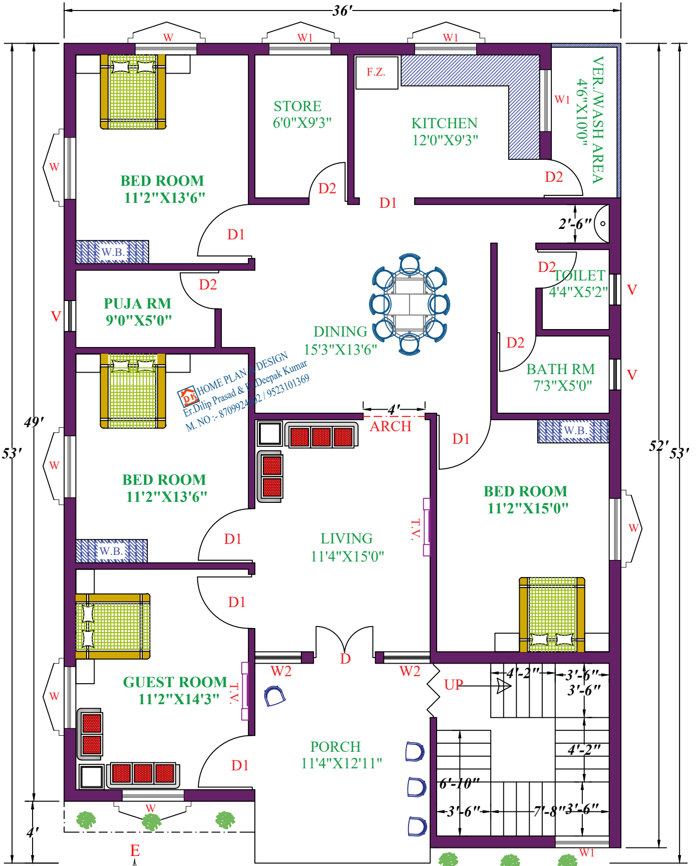
GROUND FLOOR
