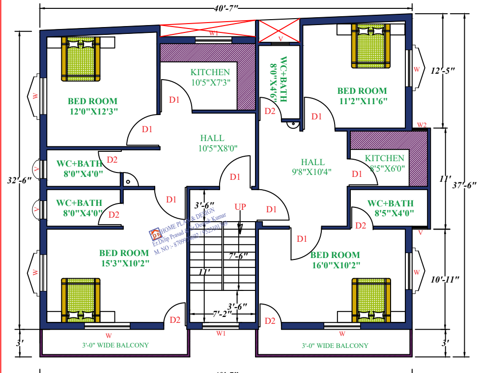
1ST FLOOR
