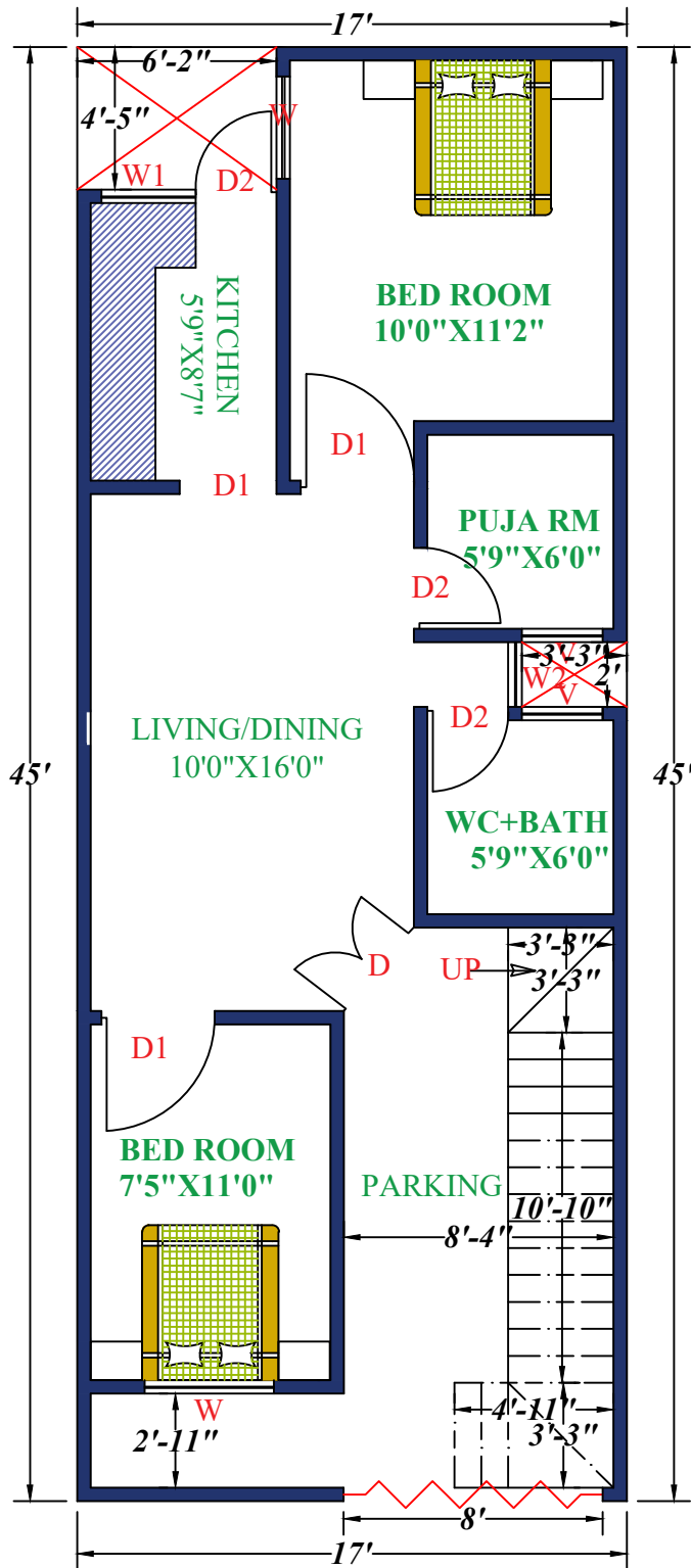
GROUND FLOOR
