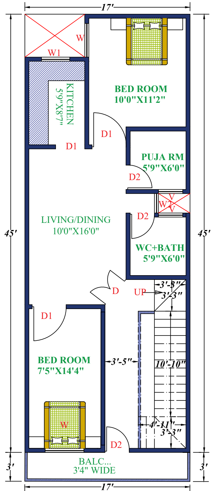
1ST FLOOR
