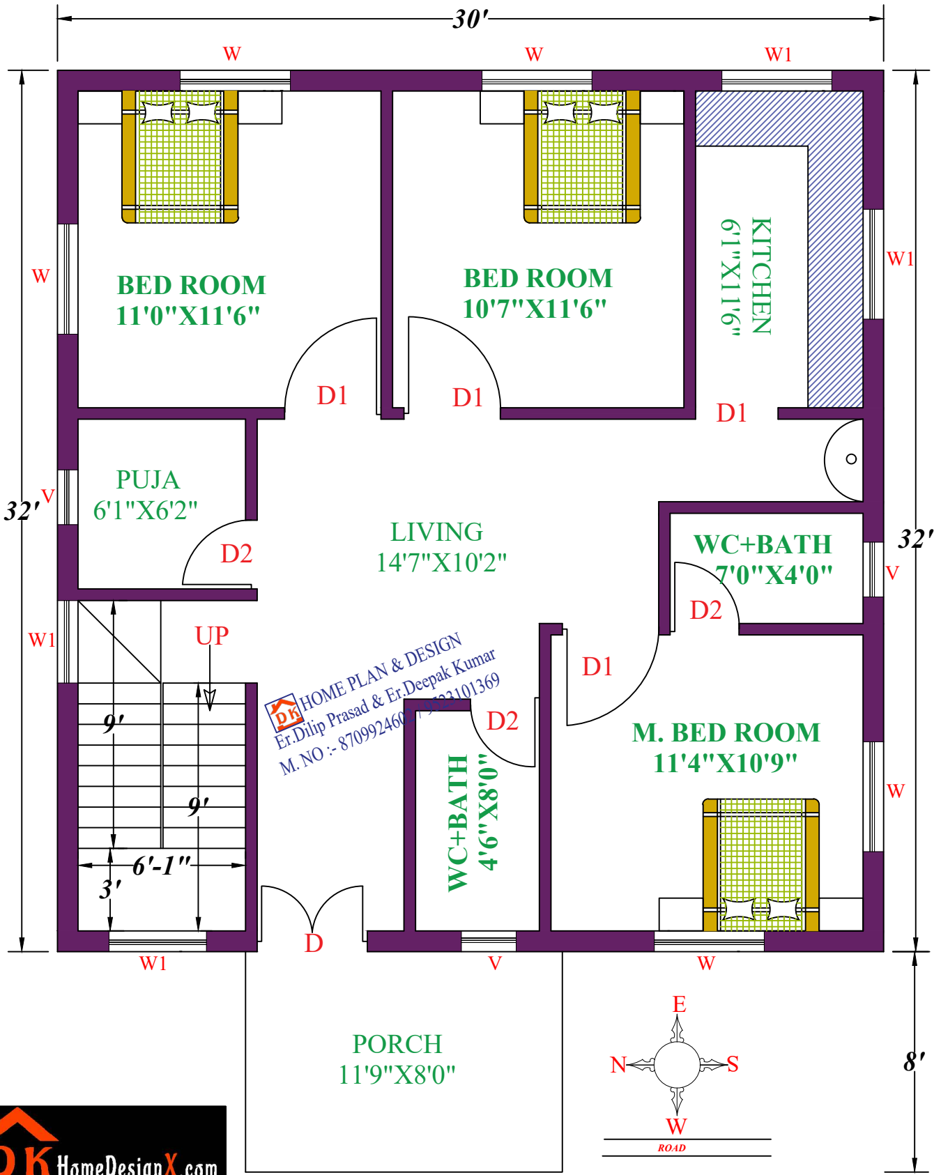
GROUND FLOOR
