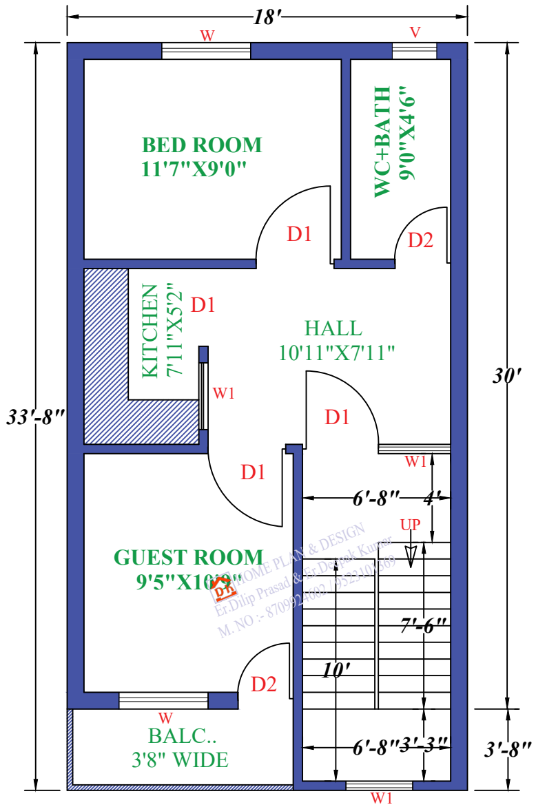
1ST FLOOR
