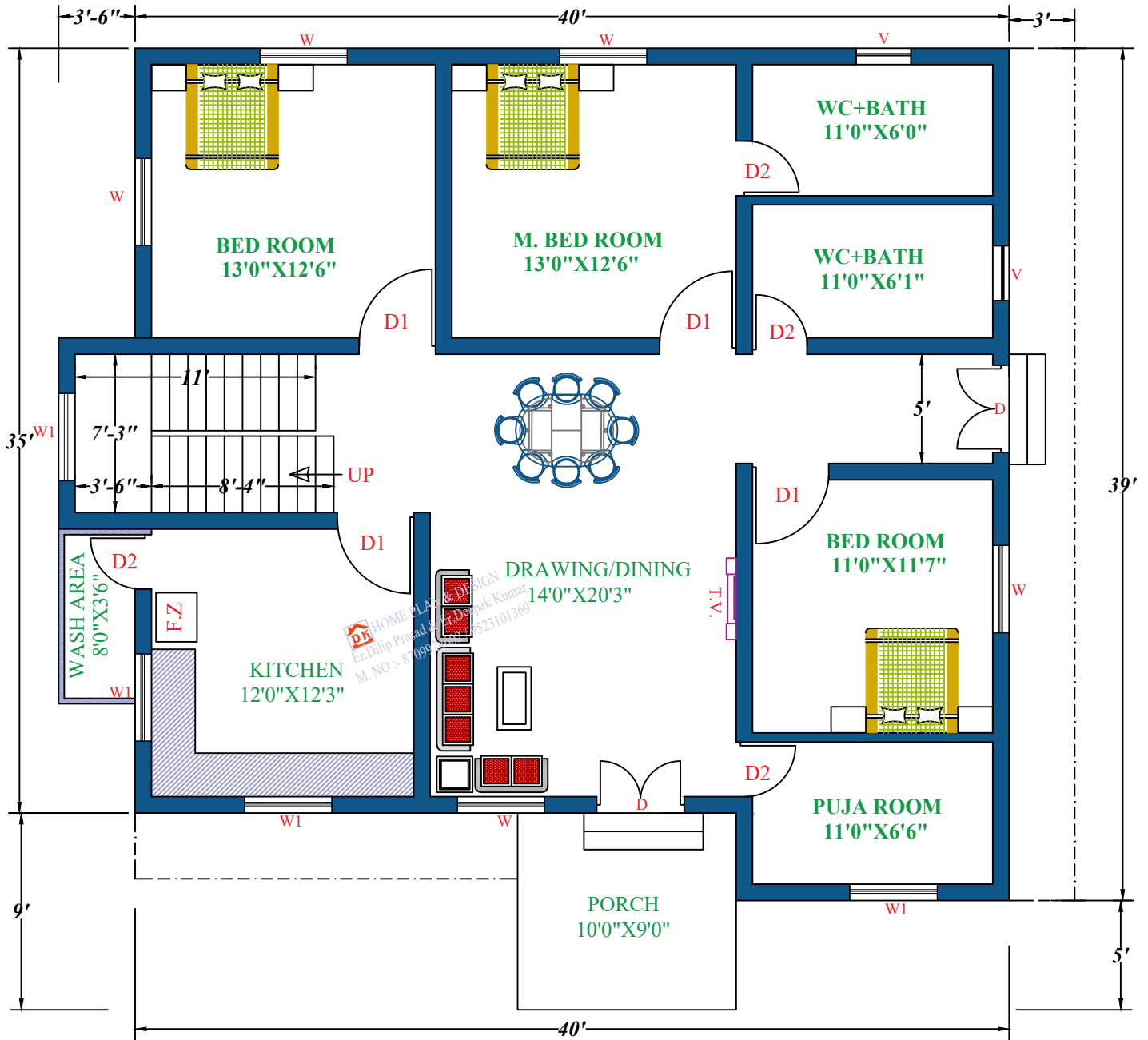
GROUND FLOOR
