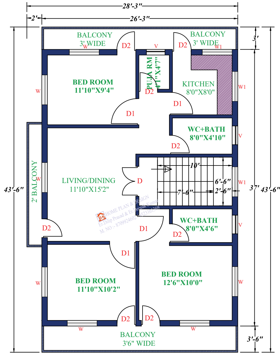
1ST FLOOR
