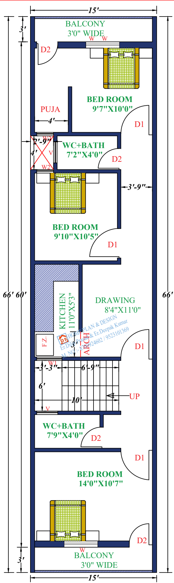
1ST FLOOR
