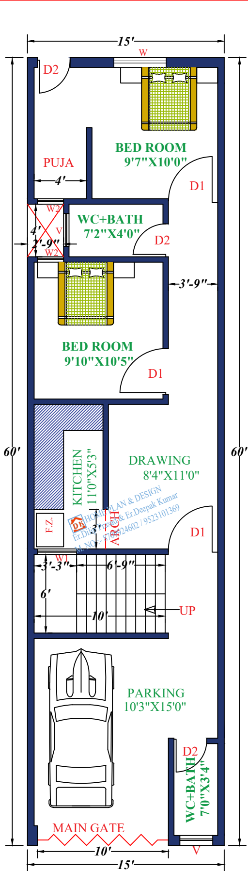
GROUND FLOOR
