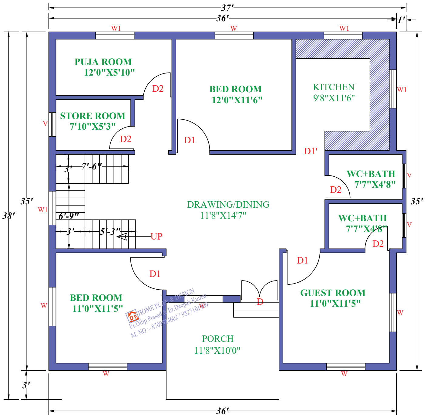
GROUND FLOOR
