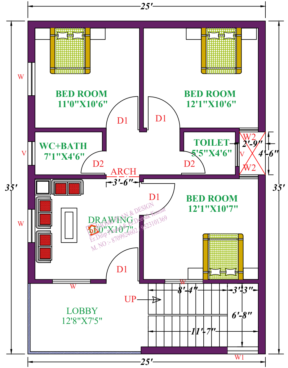
1ST & 2ND FLOOR
