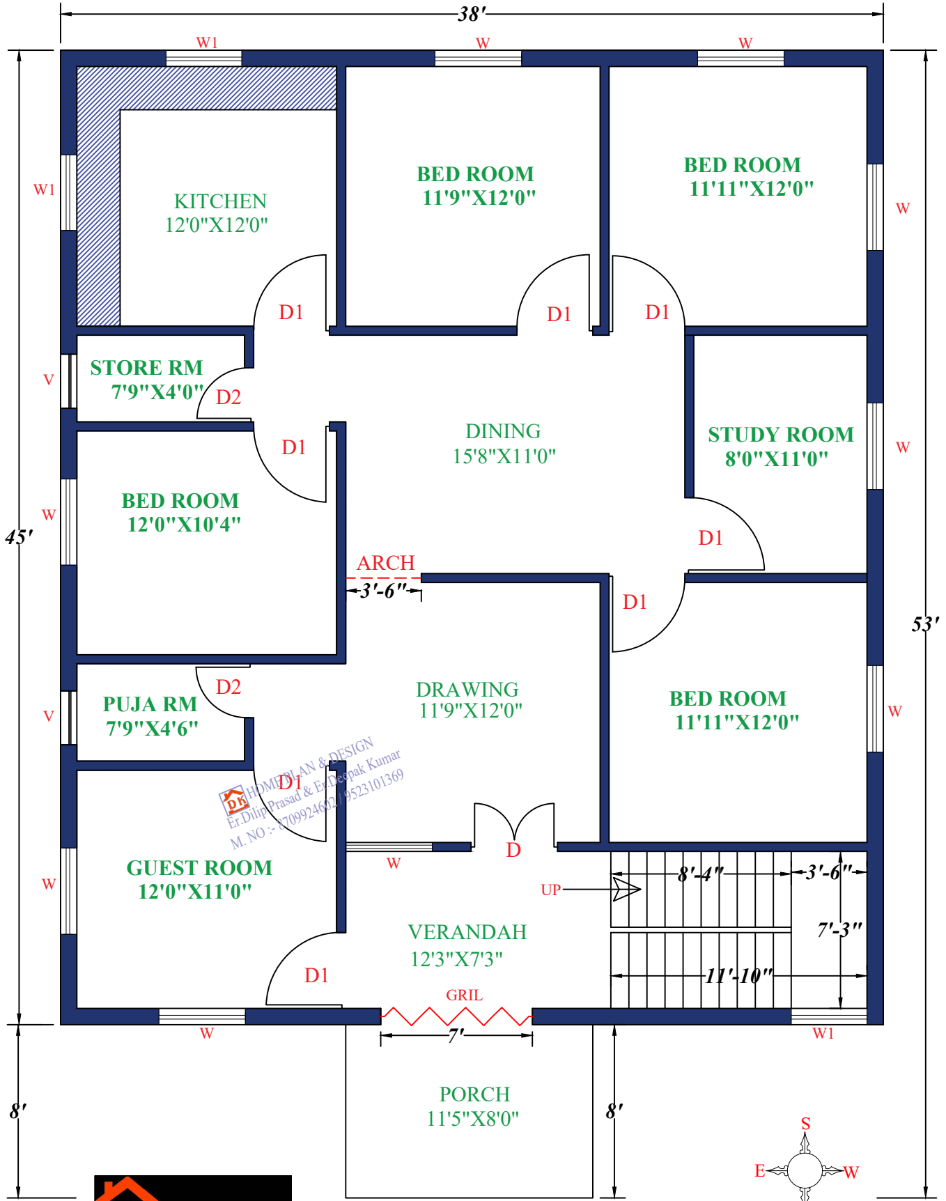
GROUND FLOOR
