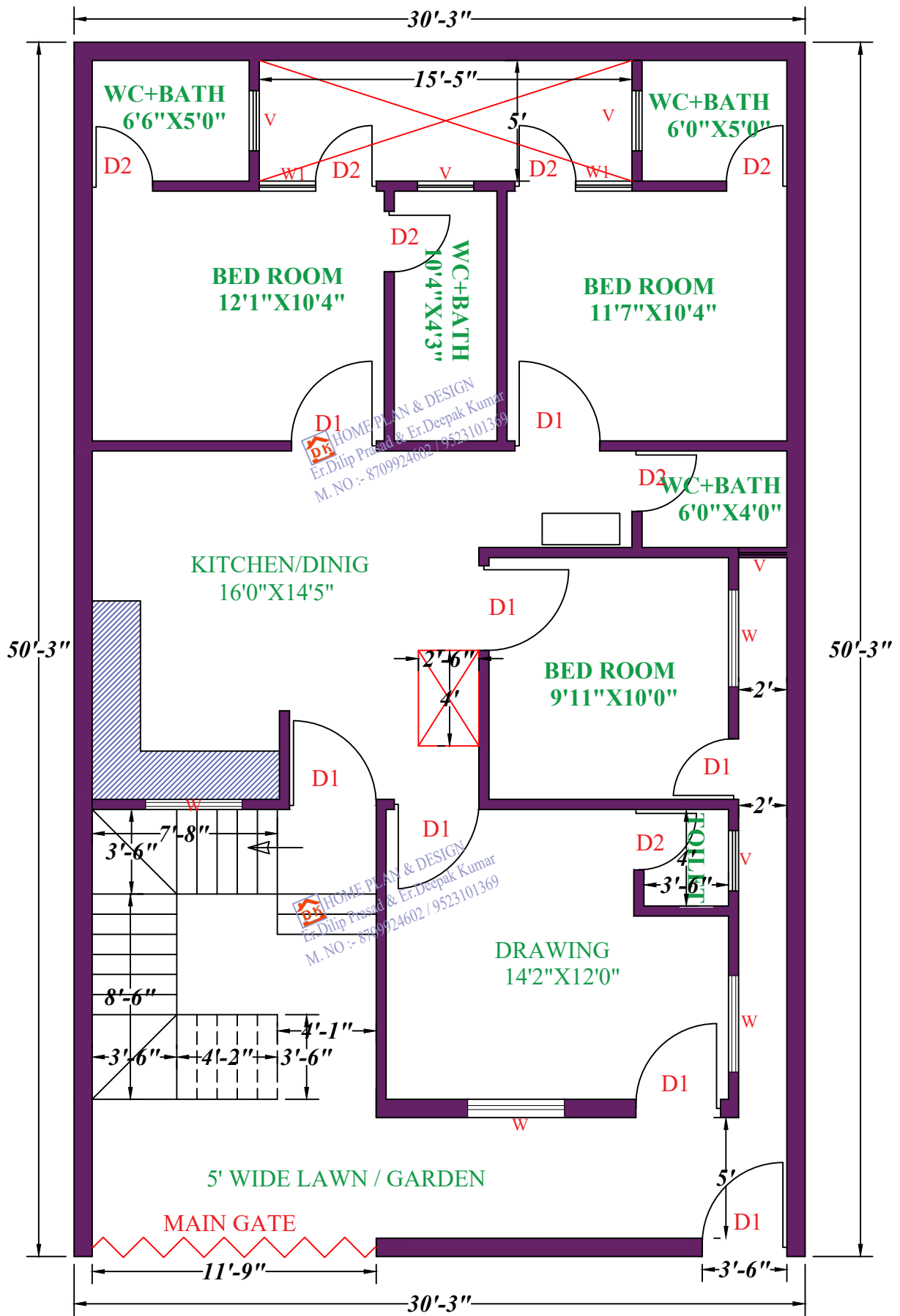
GROUND FLOOR
