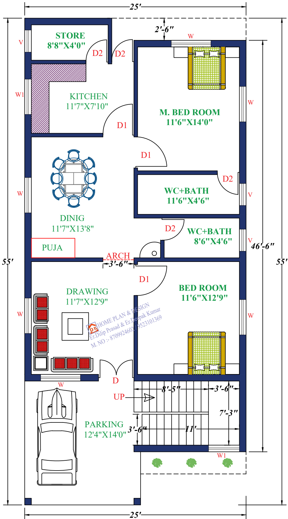
GROUND FLOOR
