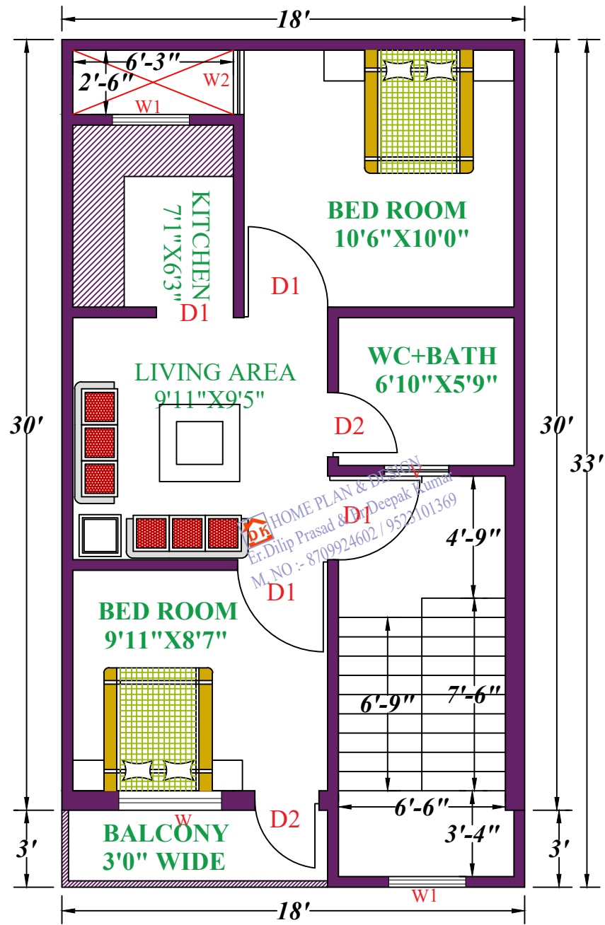
1ST FLOOR
