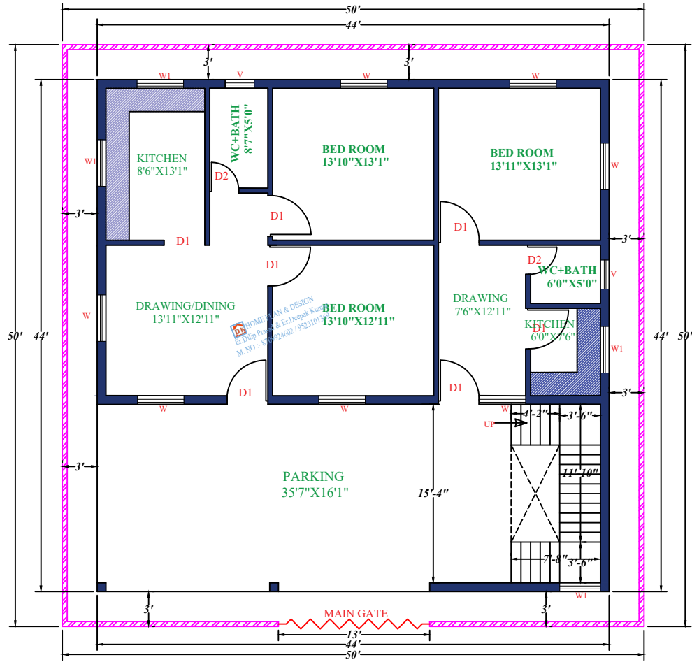
GROUND FLOOR
