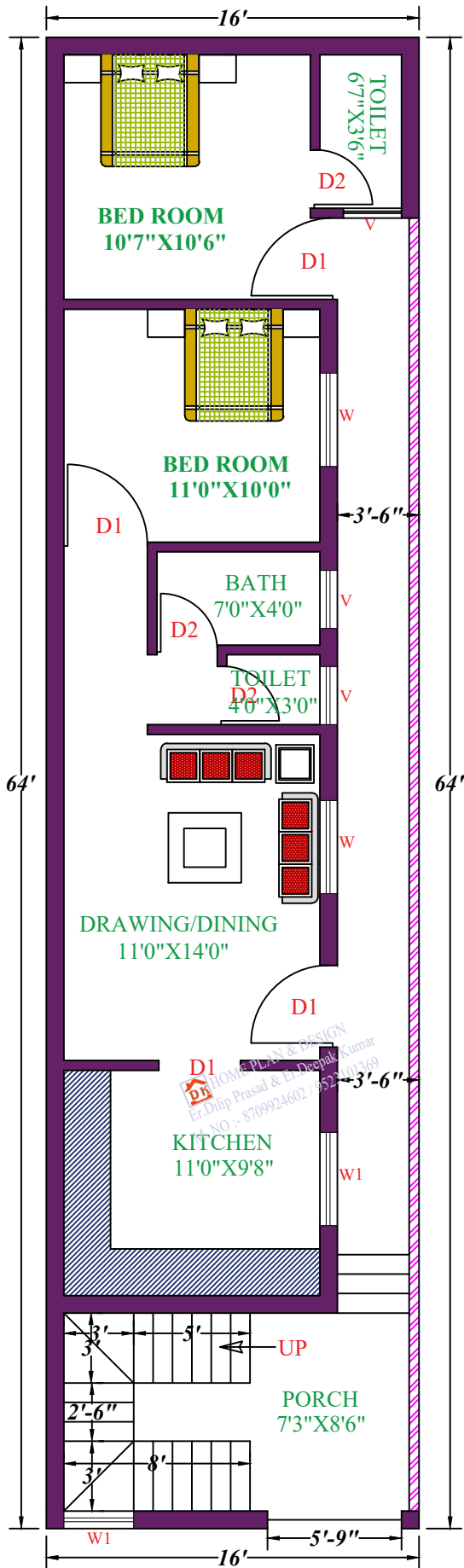
GROUND FLOOR
