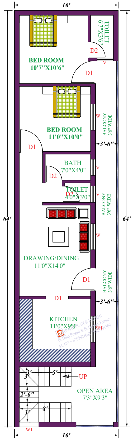
1ST FLOOR
