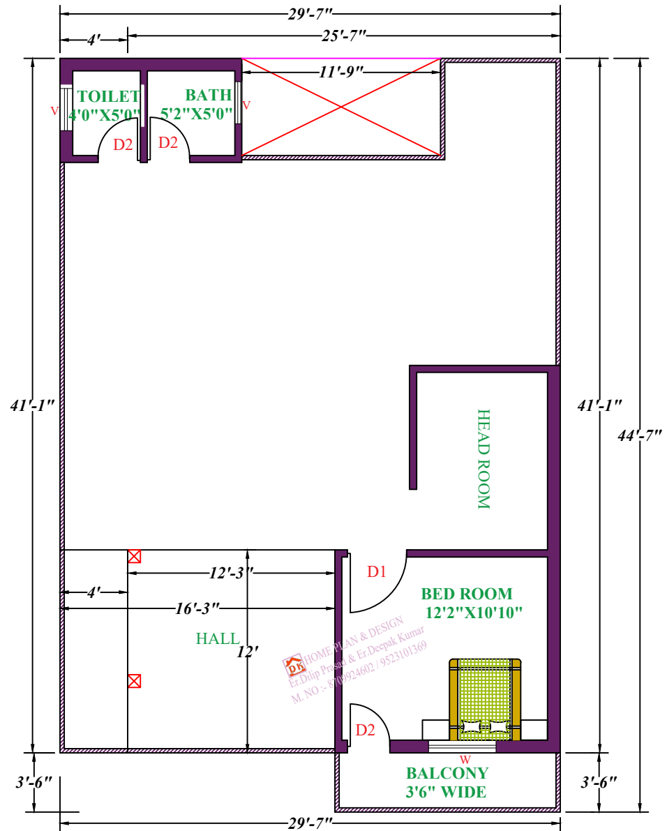
1ST FLOOR
