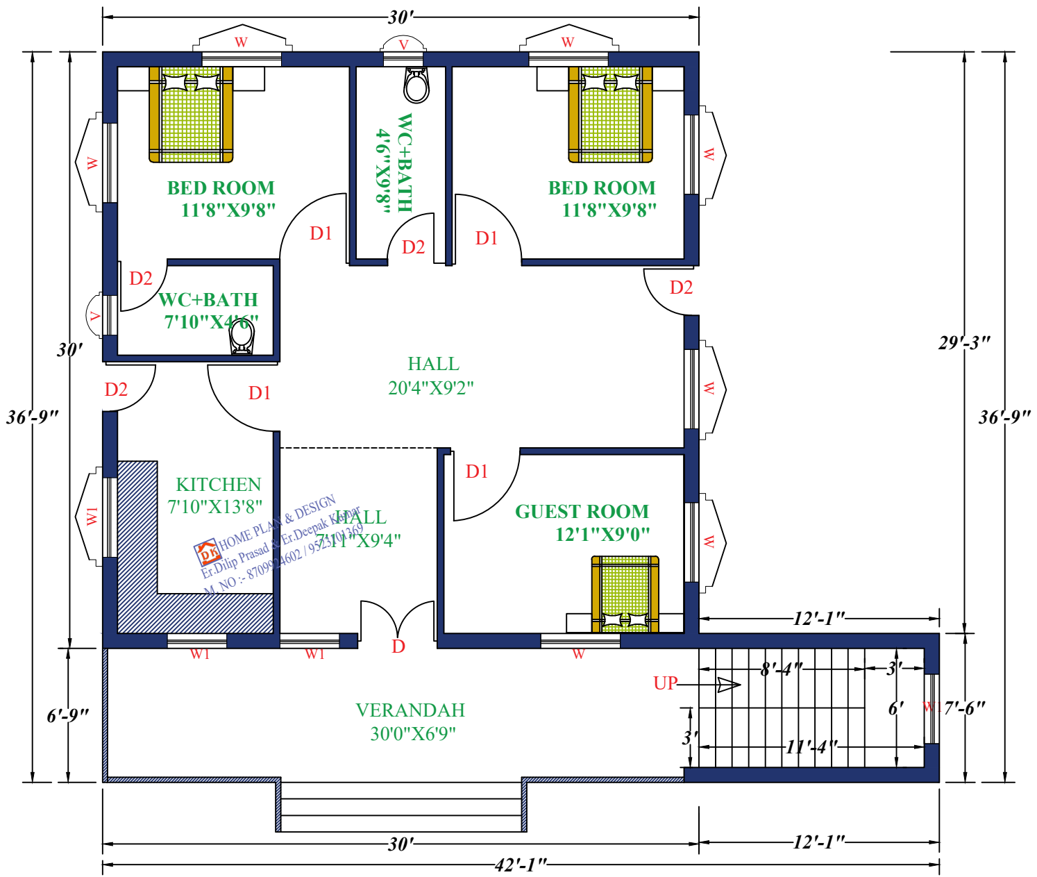
GROUND FLOOR
