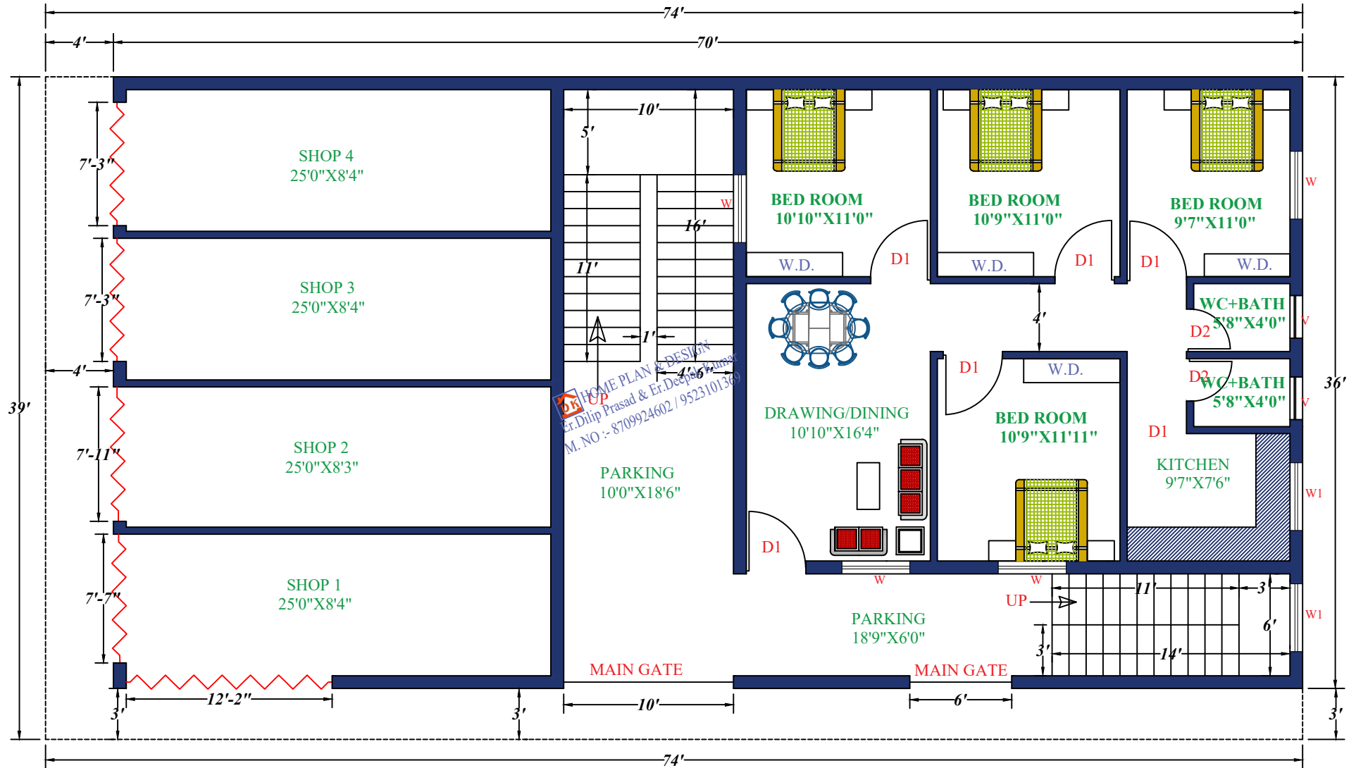
GROUND FLOOR
