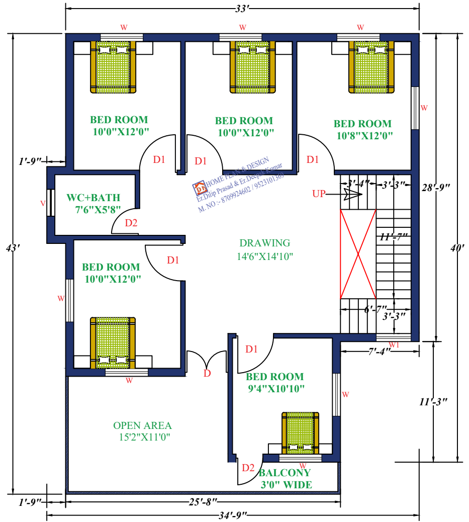
1ST FLOOR
