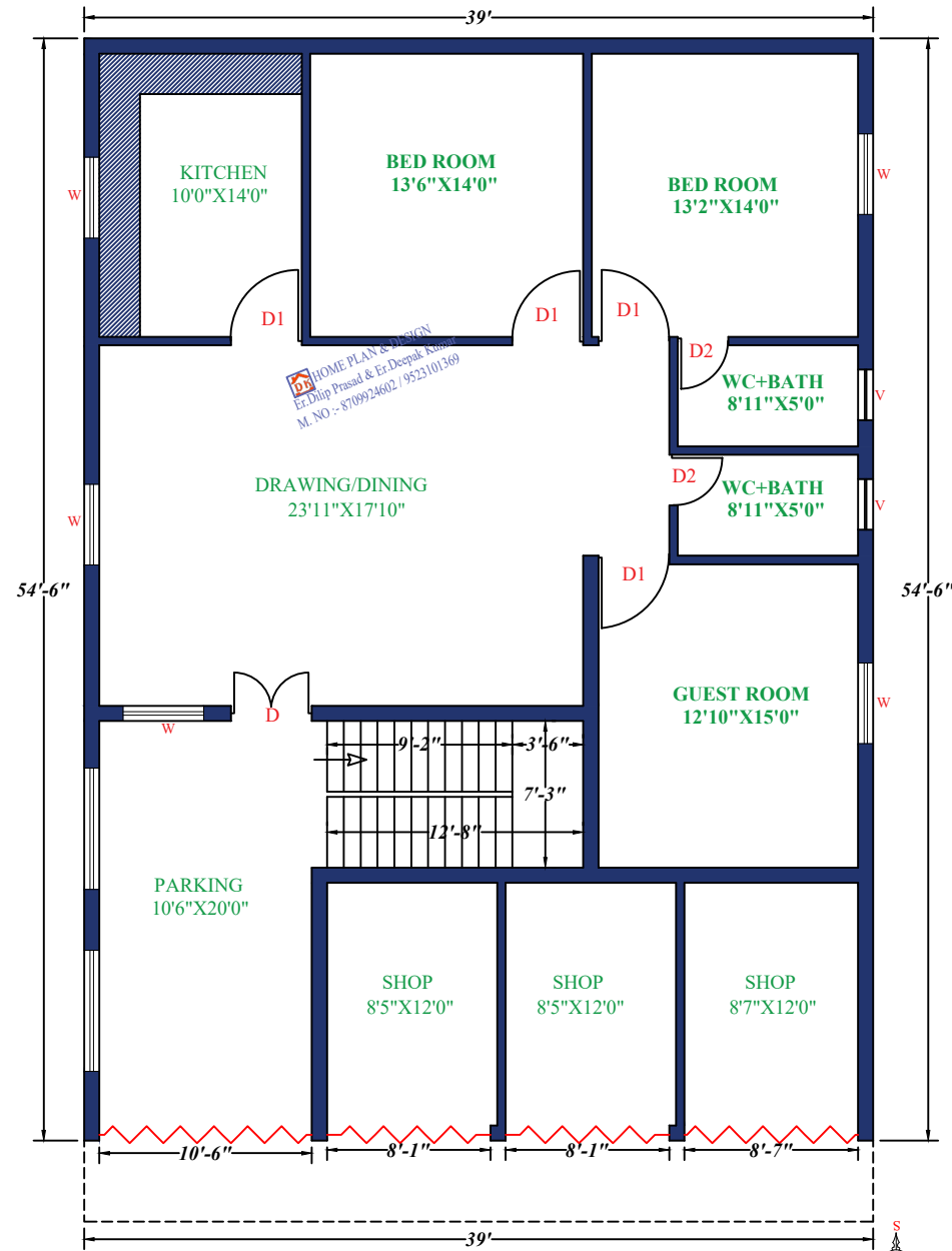
GROUND FLOOR
