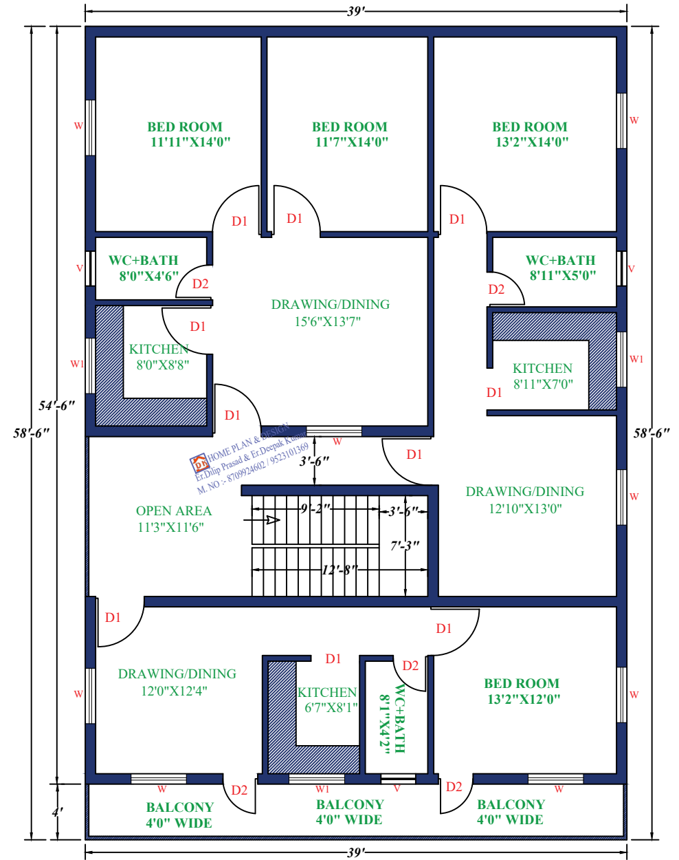
1ST FLOOR
