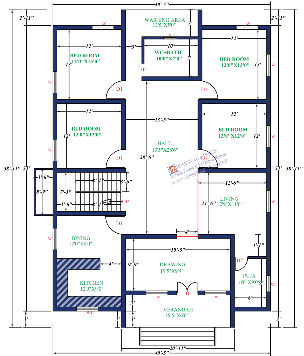
GROUND FLOOR
