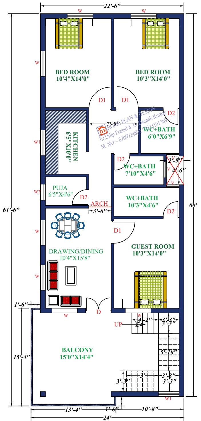
1ST FLOOR
